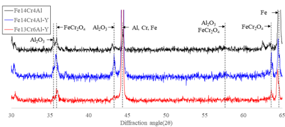
Fig. 12. Diffraction phase through HRXRD of FeCrAl alloy.
